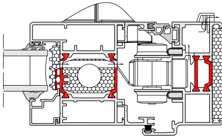
BSF70 HI CILL
