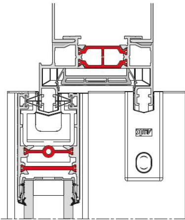
S67 DOUBLE TRACK HEAD
