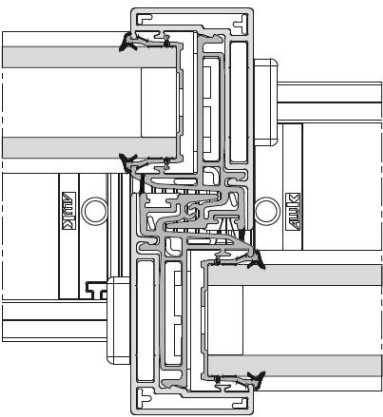
S67 DOUBLE TRACK / TRIPLE TRACK INTERLOCK
