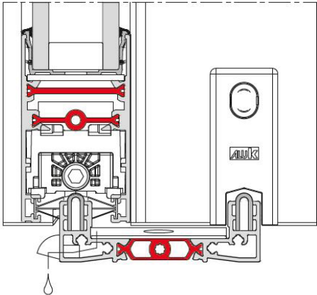
S67 DOUBLE TRACK LOW THRESHOLD
