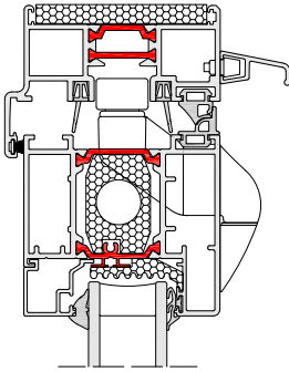
BSF70 HI HEAD
