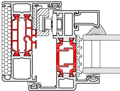
HERITAGE DOOR OPEN OUT LOCK JAMB
