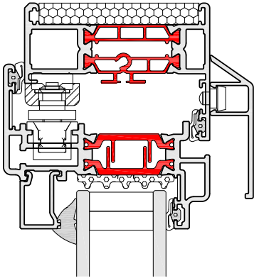
HERITAGE DOOR OPEN OUT CILL
